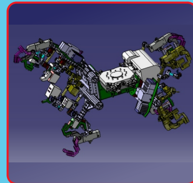
EGP TYPE HANDLING GRIPPER FOR DOOR INNER ASSY
