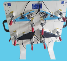
Checking Fixture For Cheater for U321
