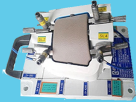
Fixture for Tail Gate Cap For U321
