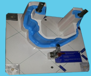
Checking Fixture for Fuse Box
