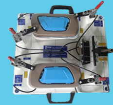
Fixture For Bezel Release Handle Bag for U321
