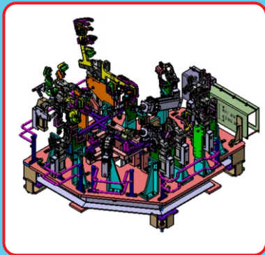
SPOT WELDING FIXTURE FOR DOOR INNER SUB ASSY
